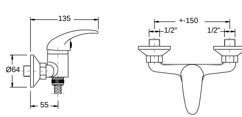
02. Monocomando de base chuveiro Wall mounted tap for shower tray Mitigeur de douche
