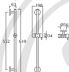
07.Rampa chuveiro | Shower rail | Barre de Douche
