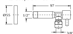
16. Tomeira esquadria 1/2" x 3/8" 1/2" x 3/8" Tap Robinete d'équerre 1/2" x 3/8" Assi
