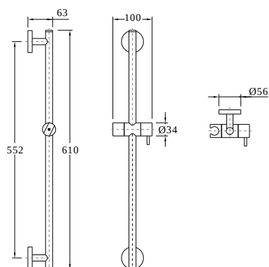
07.Rampa chuveiro | Shower rail | Barre de Douche
